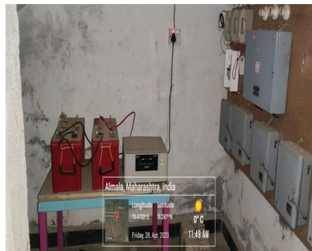
INVERTER ROOM
